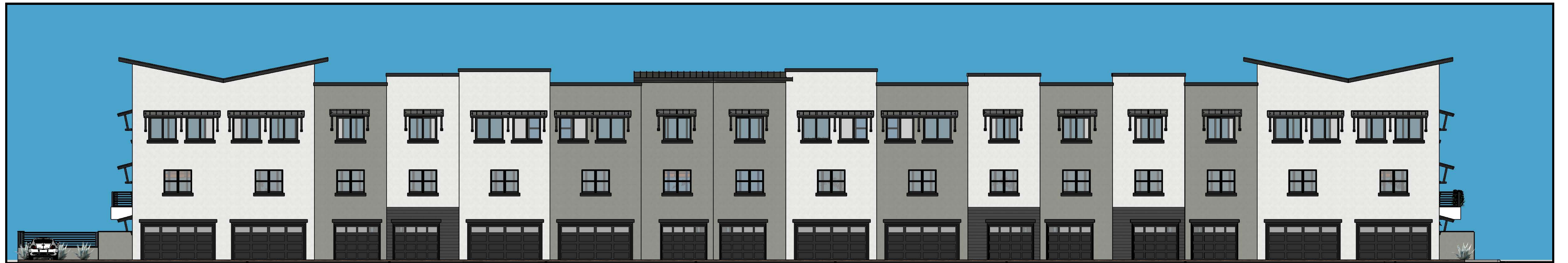
Building B South Elevation Scale: 1"=10'
