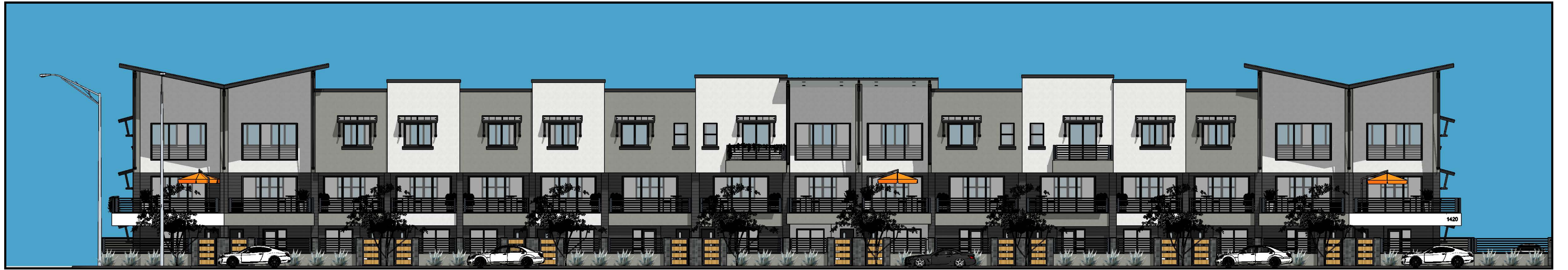
Building B North Elevation Scale: 1"=10'
